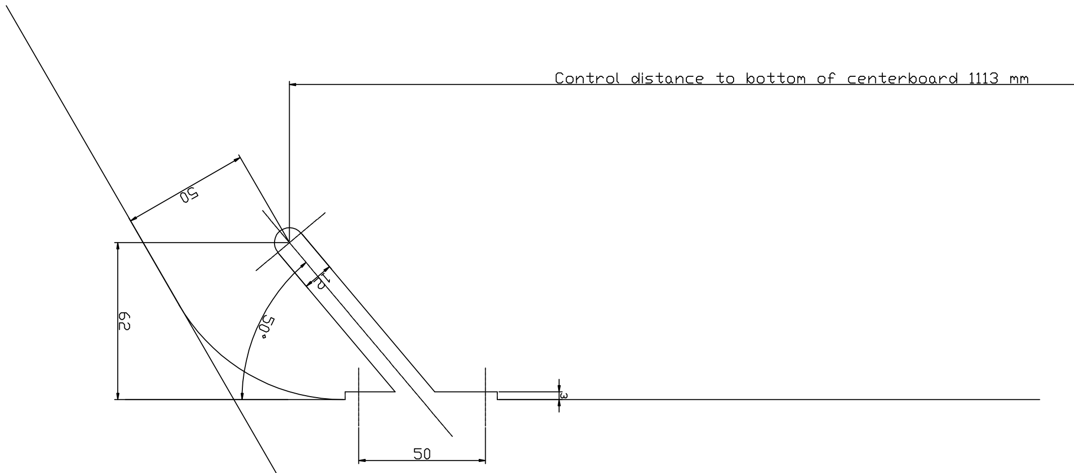
Wayfarer MK IV Centerboard. Cut-out for pivot bolt. Measures taken from centerboard from W 11225. jan. 2019 - Jens Konge
